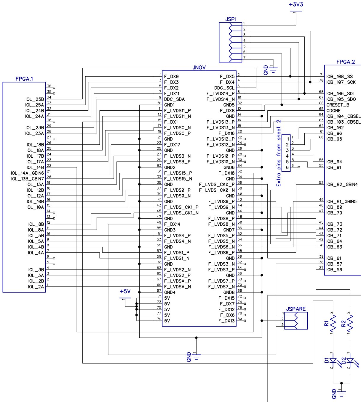
Spare I/O not routed between FPGAs
